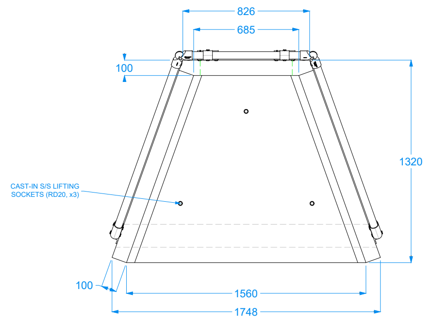
VIEW: TOP
