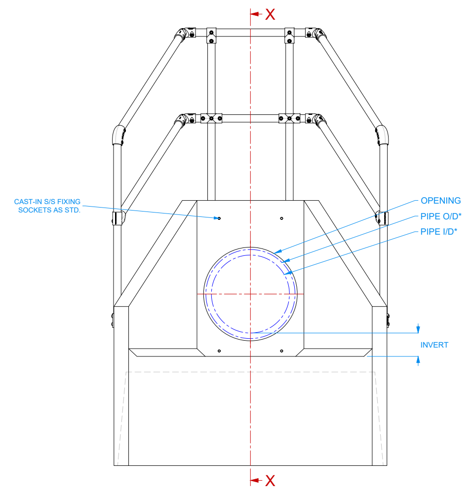
VIEW: FRONT
